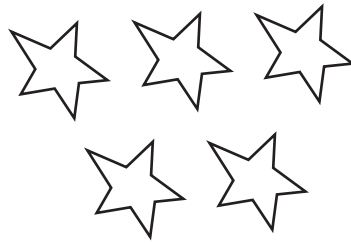
Constellation
